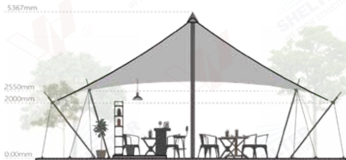
剖面圖 Sectional View
