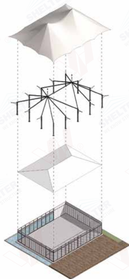
爆炸圖 Exploded View
