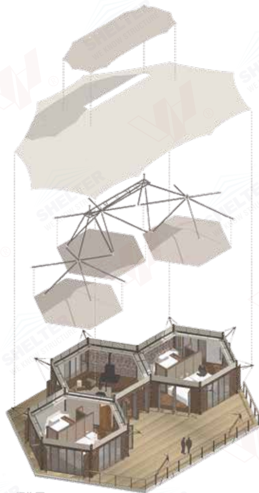
爆炸圖 Exploded View
